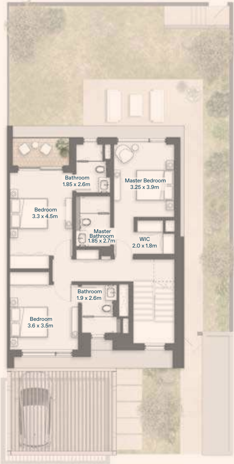
First Floor
